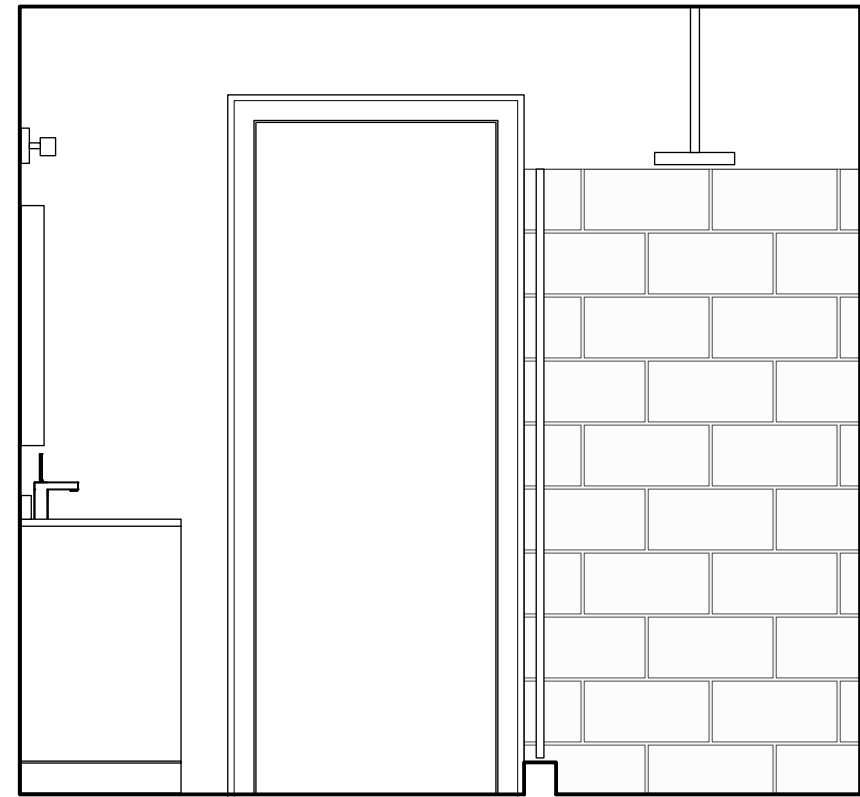
8 MASTER BATH INTERIOR ELEVATION SCALE= 1/2" = 1'-0"
