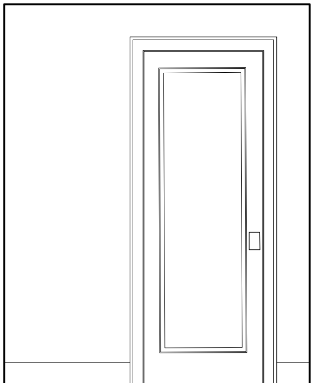
11 POWDER INTERIOR ELEVATION SCALE= 1/2" = 1'-0"
