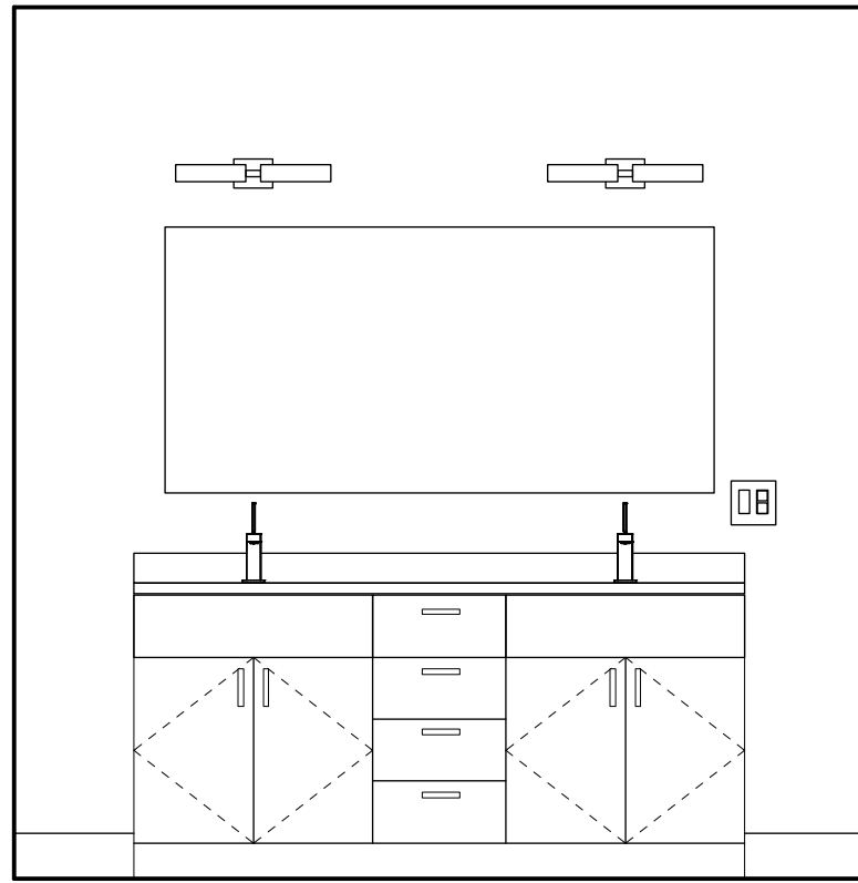
5 MASTER BATH INTERIOR ELEVATION SCALE= 1/2" = 1'-0"
