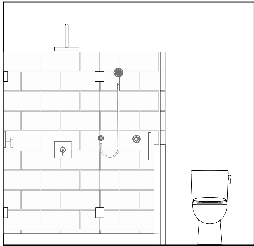
6 MASTER BATH INTERIOR ELEVATION SCALE= 1/2" = 1'-0"
