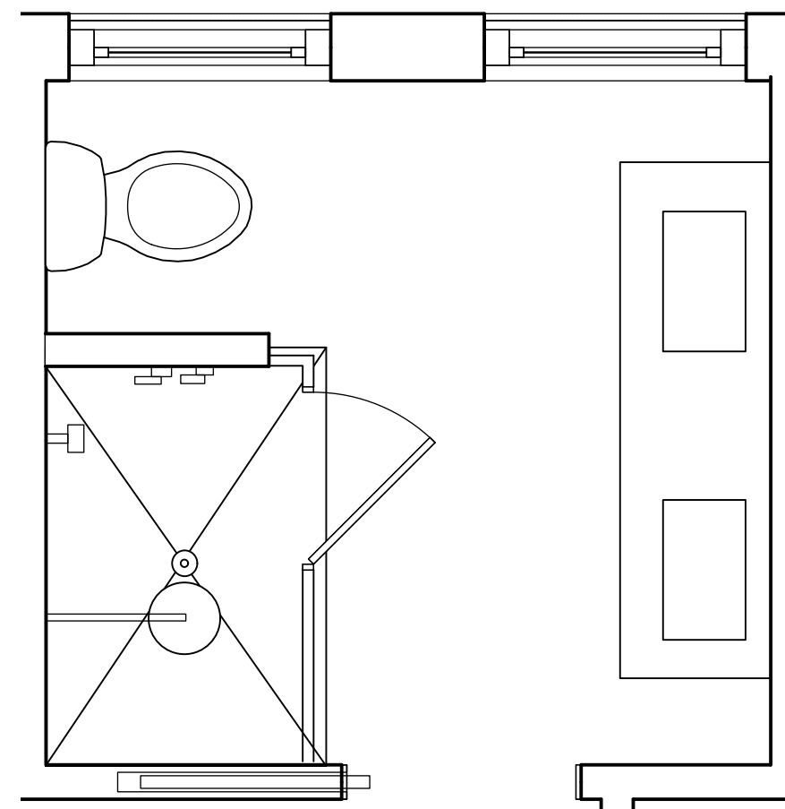
13 MASTER BATH PLAN SCALE= 1/2" = 1'-0"
