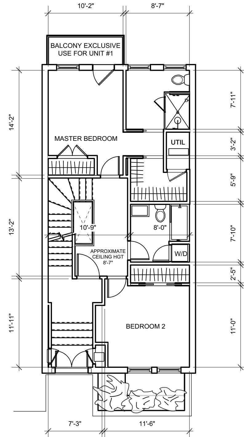
PARLOR & GARDEN DUPLEX UNIT #1 PARLOR LEVEL APPROXIMATELY 695 SQ.FT.
