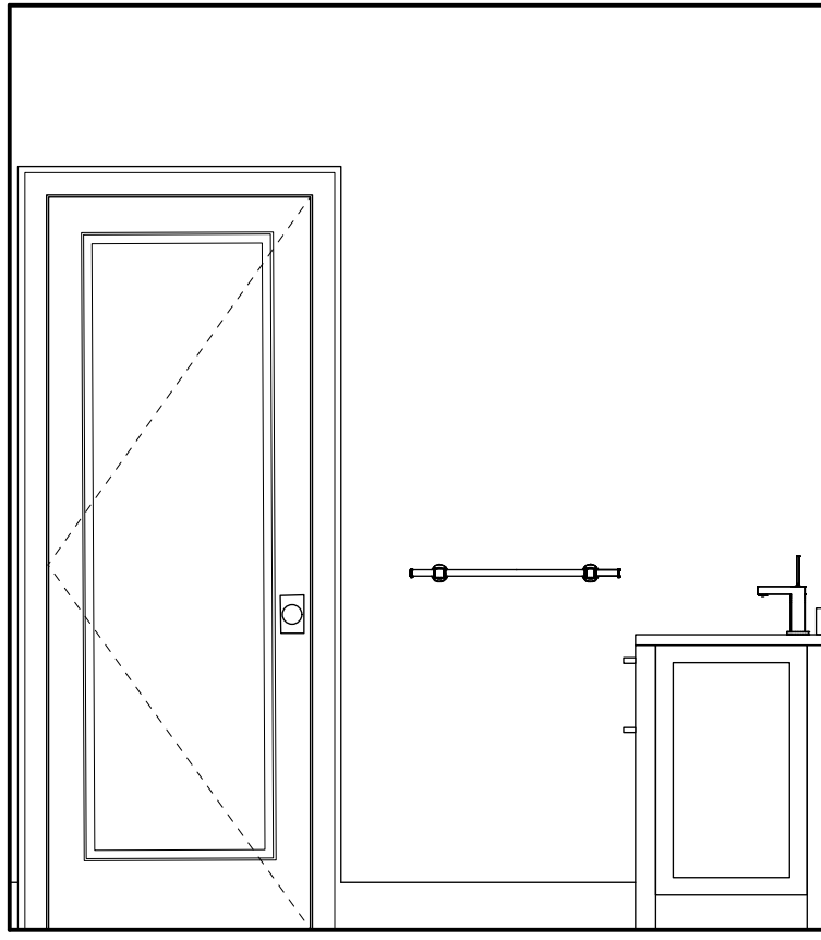
6 INTERIOR ELEVATION SCALE= 1/2" = 1'-0"
