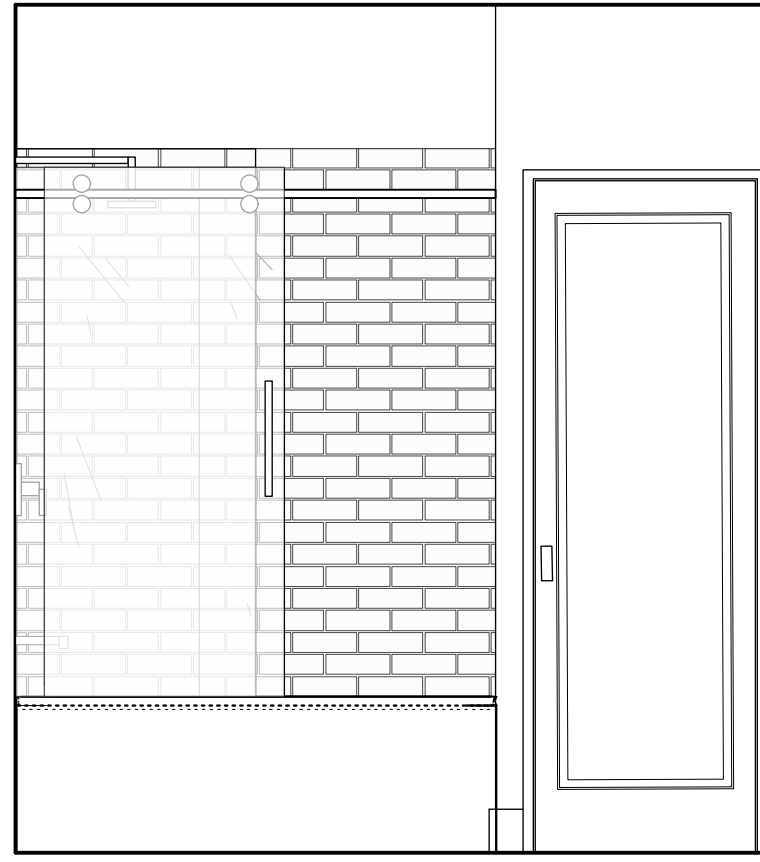
7 INTERIOR ELEVATION SCALE= 1/2" = 1'-0"
