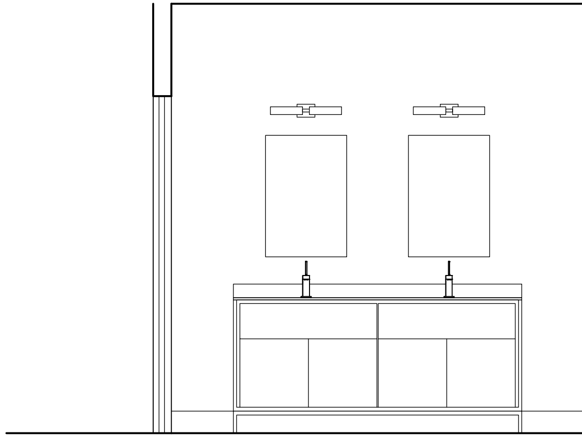
2 INTERIOR ELEVATION SCALE= 1/2" = 1'-0"
