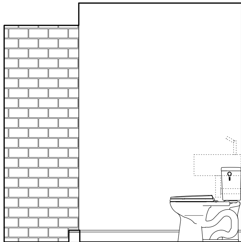
11 INTERIOR ELEVATION SCALE= 1/2" = 1'-0"
