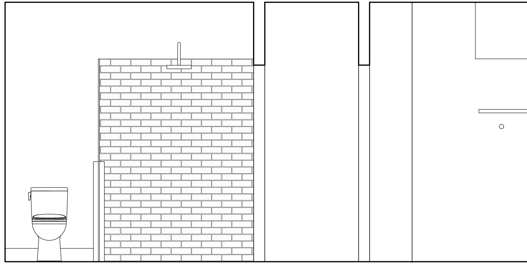
3 INTERIOR ELEVATION SCALE= 1/2" = 1'-0"
