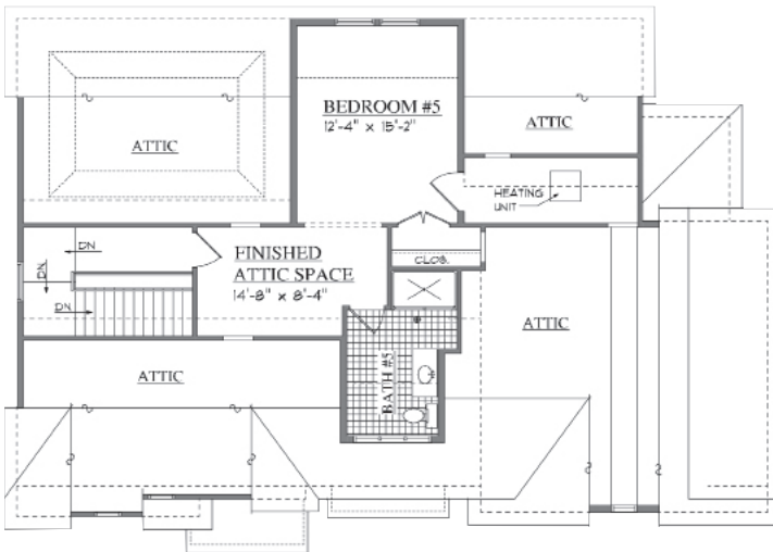
third floor
